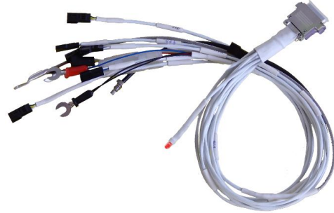
UAV ECU and Harness
